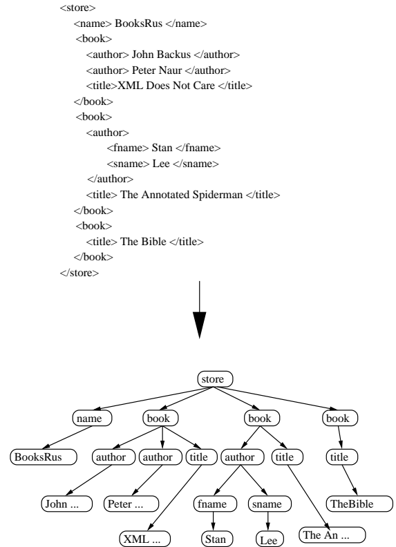
Figure 1: XML Parsing.
