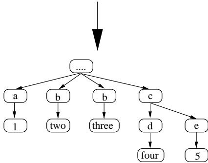
Figure 2: Encoding example.
