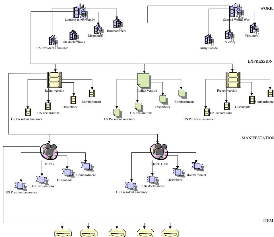
Figure 2: Running example
